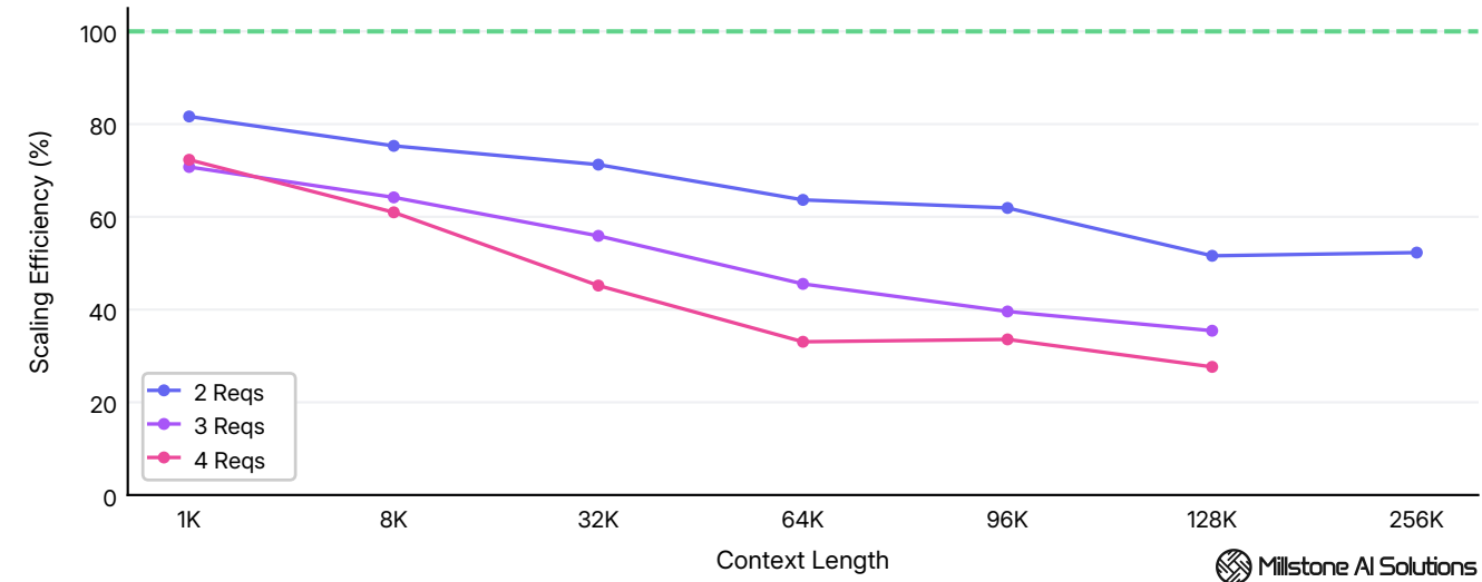
Scaling efficiency across 1K - 256K tokens context at 1 - 4 concurrent requests.
