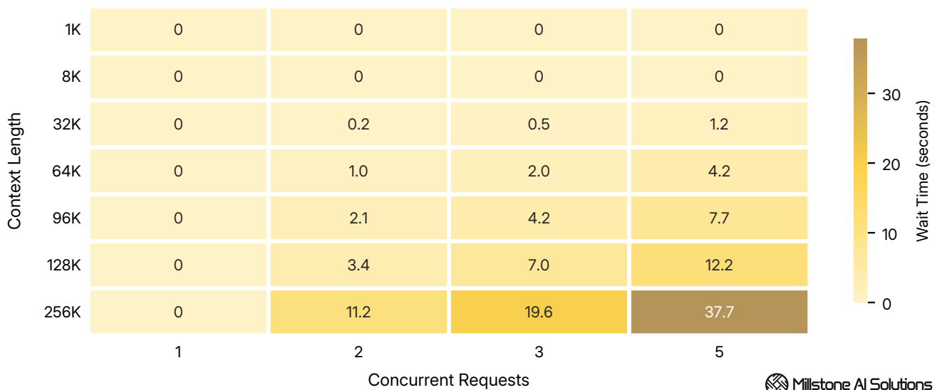
Average queue wait time across 1K - 256K tokens context at 1 - 5 concurrent requests.
