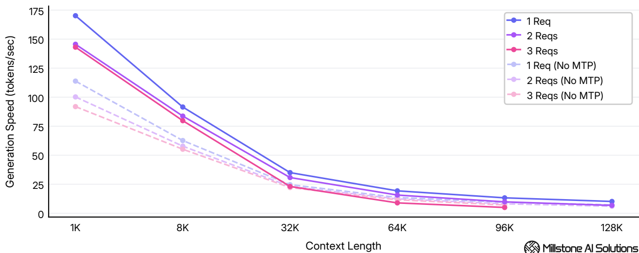
Average per-user generation speed across 1K - 128K tokens context lengths at 1 - 3 concurrency levels (No MTP shown as dashed lines).
