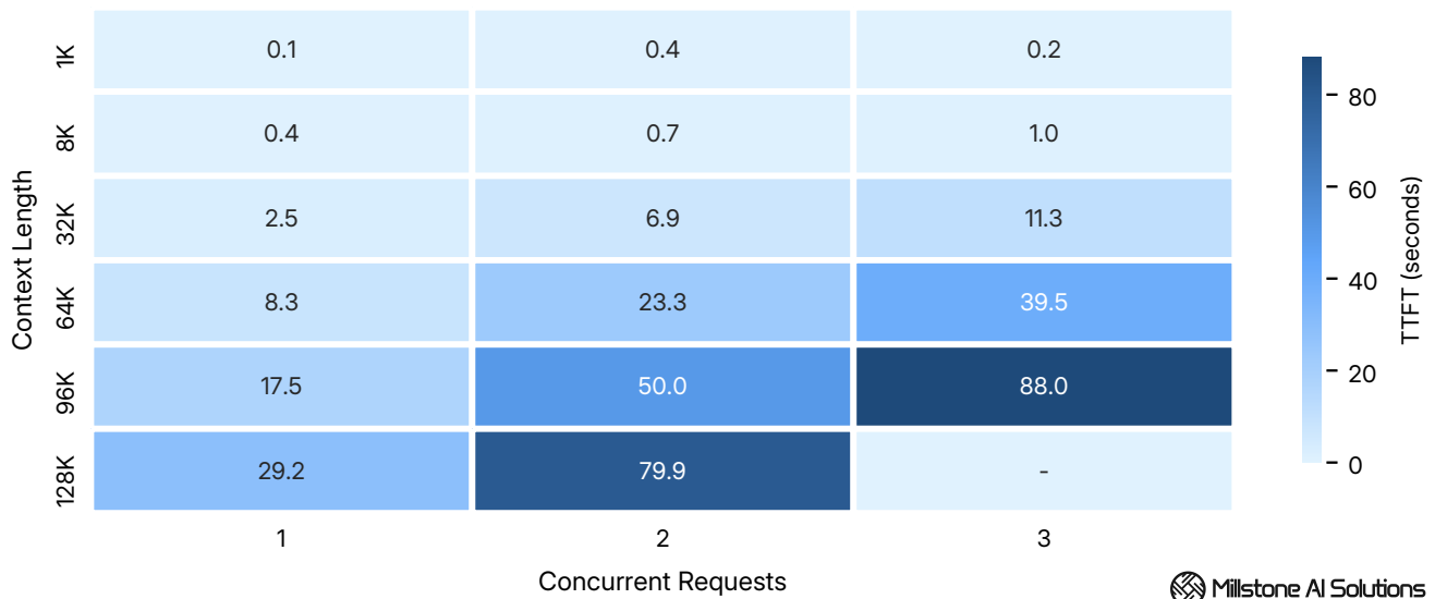
Average time to first token across 1K - 128K tokens context lengths at 1 - 3 concurrency levels.
