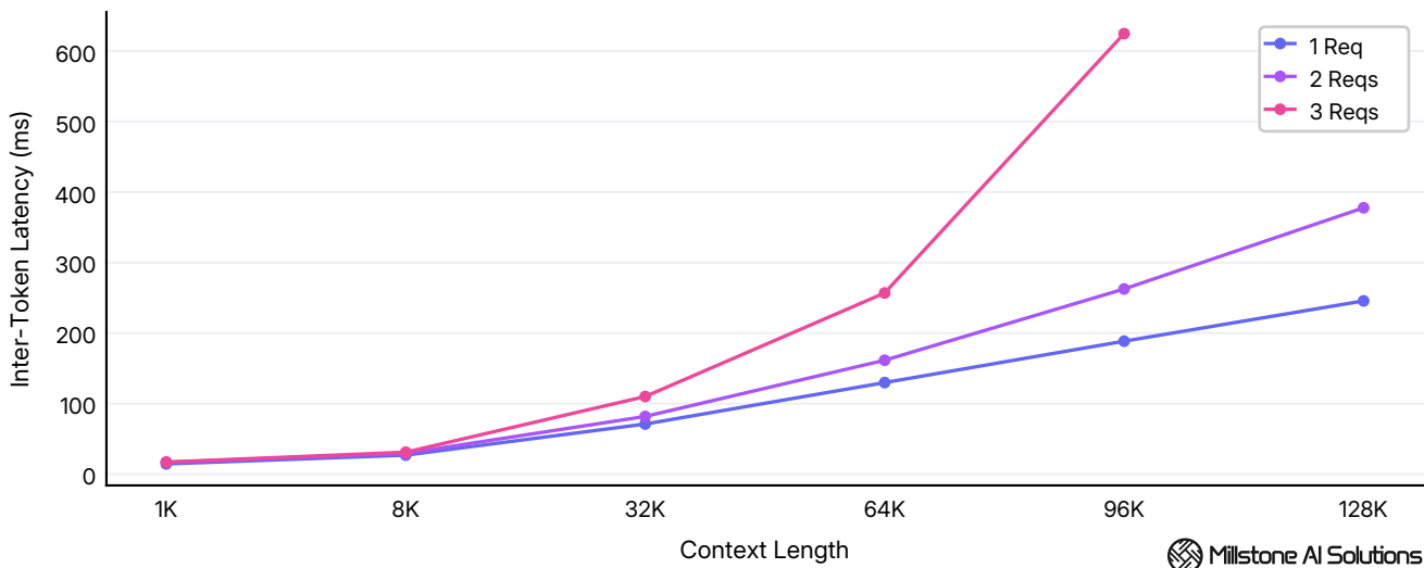
Average inter-token latency across 1K - 128K tokens context at 1 - 3 concurrent requests.
