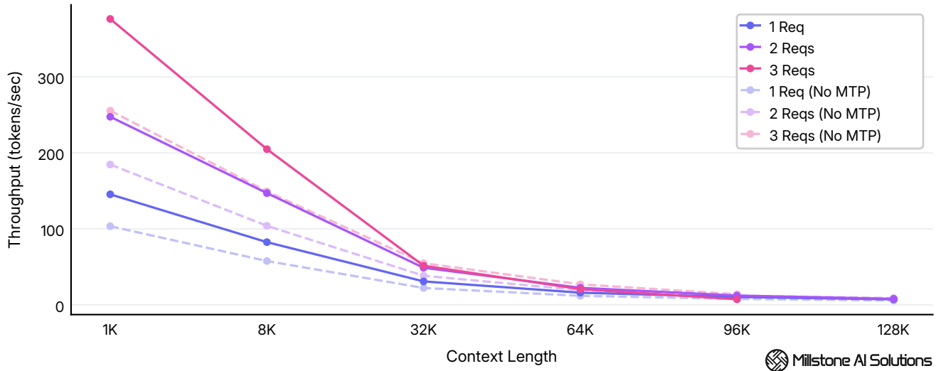
Average system throughput across 1K - 128K tokens context lengths at 1 - 3 concurrency levels (No MTP shown as dashed lines).
