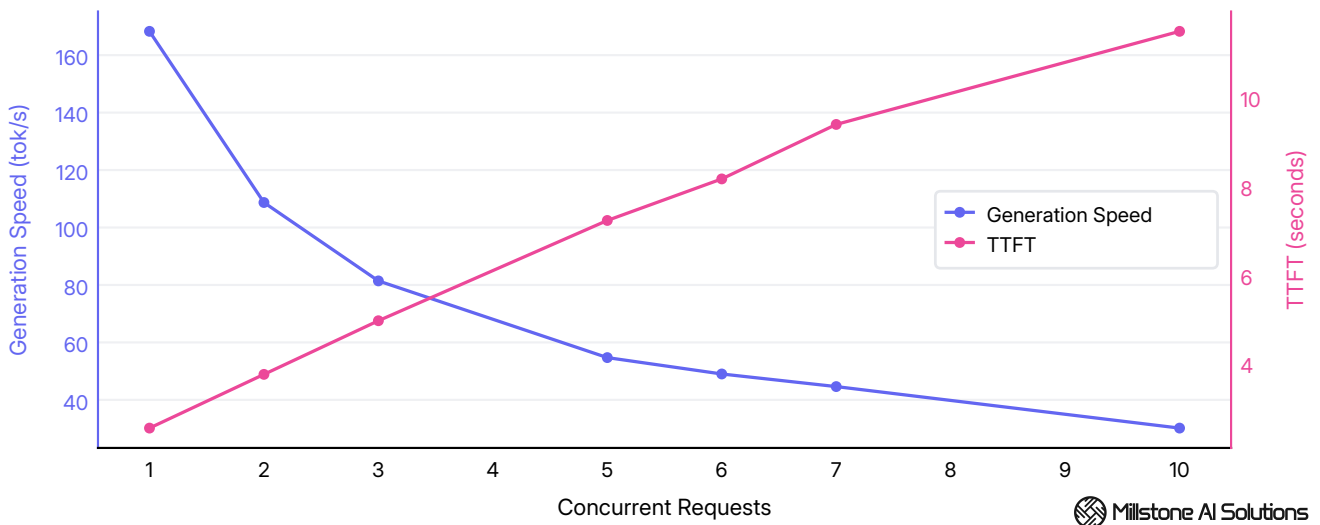
Average per-user generation speed and TTFT at 64K context.
