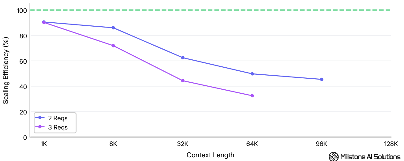
Scaling efficiency across 1K - 96K tokens context at 1 - 3 concurrent requests.
