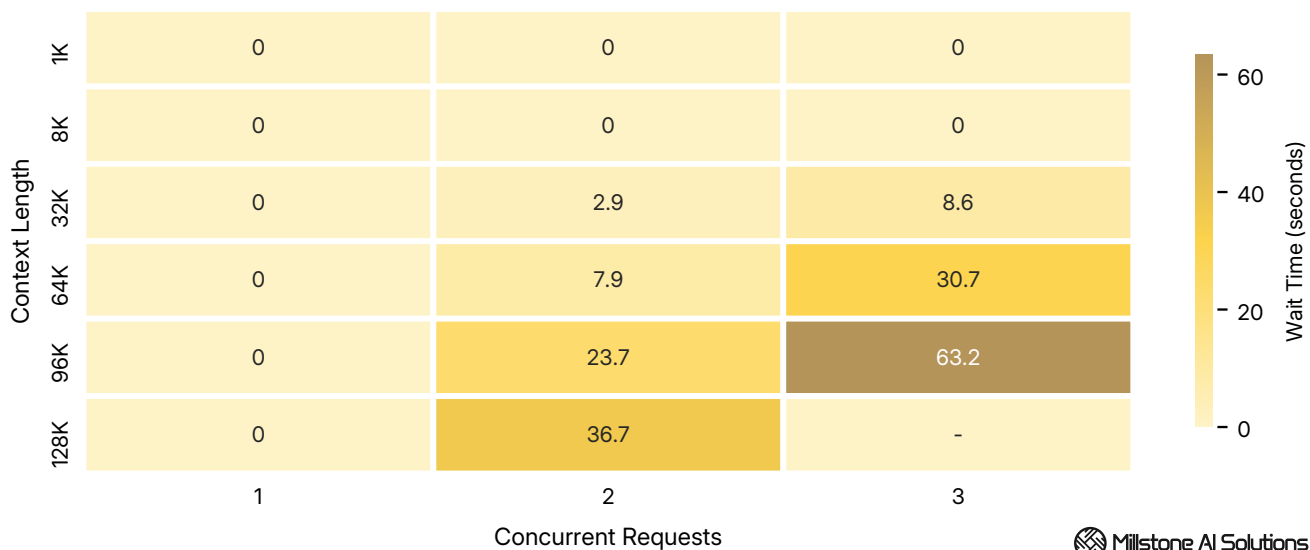
Average queue wait time across 1K - 128K tokens context at 1 - 3 concurrent requests.
