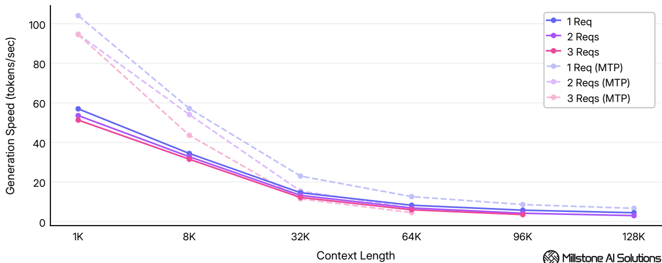
Average per-user generation speed across 1K - 128K tokens context lengths at 1 - 3 concurrency levels (MTP shown as dashed lines).
