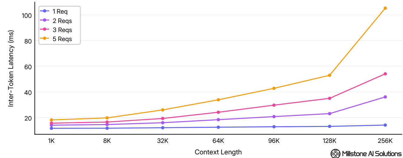
Average inter-token latency across 1K - 256K tokens context at 1 - 5 concurrent requests.
