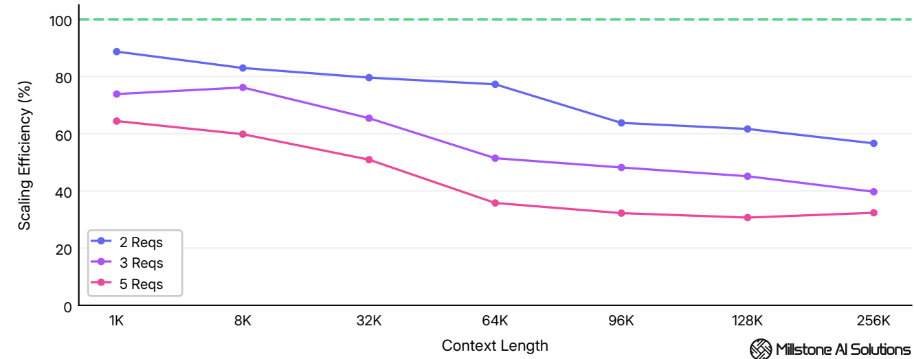
Scaling efficiency across 1K - 256K tokens context at 1 - 5 concurrent requests.
