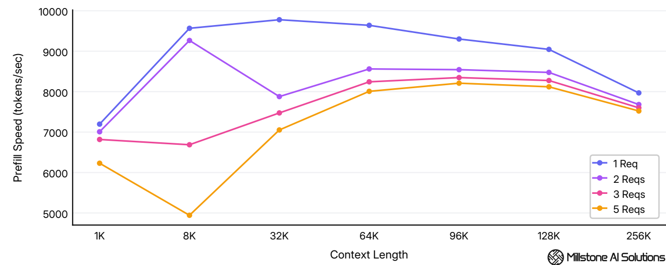
Average per-user prefill speed across 1K - 256K tokens context at 1 - 5 concurrent requests.
