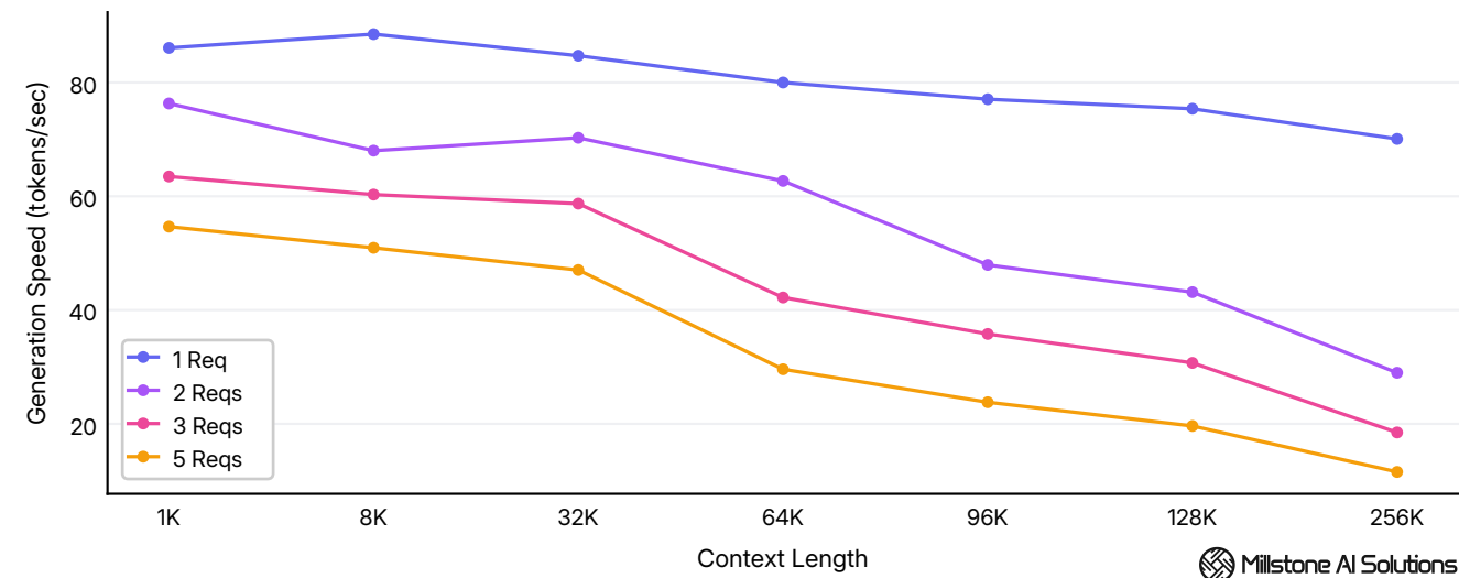
Average per-user generation speed across 1K - 256K tokens context lengths at 1 - 5 concurrency levels.
