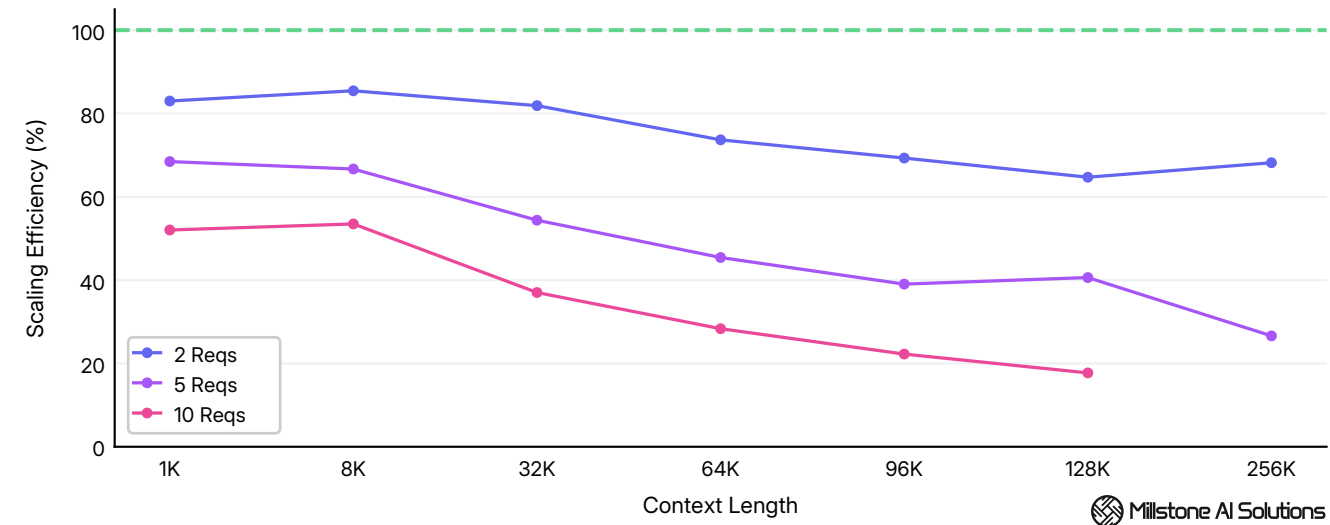
Scaling efficiency across 1K - 256K tokens context at 1 - 10 concurrent requests.
