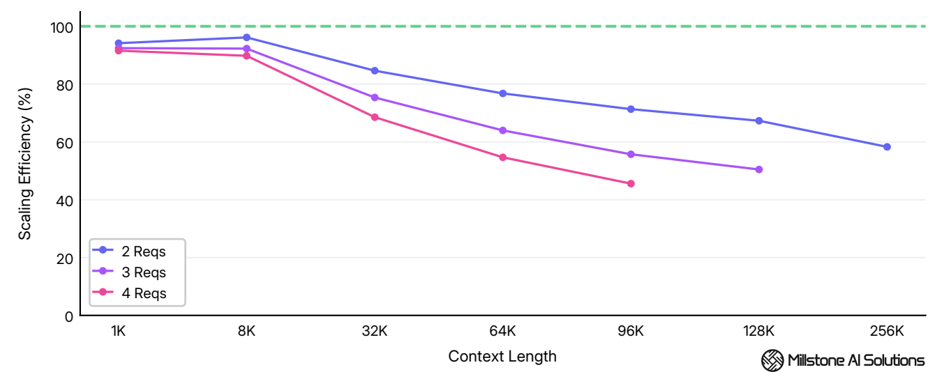
Scaling efficiency across 1K - 256K tokens context at 1 - 4 concurrent requests.
