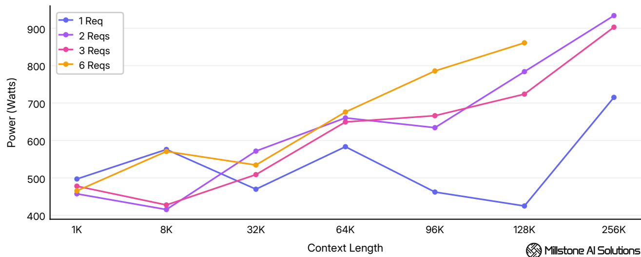
Average GPU power draw across 1K - 256K tokens context at 1 - 6 concurrent requests.
