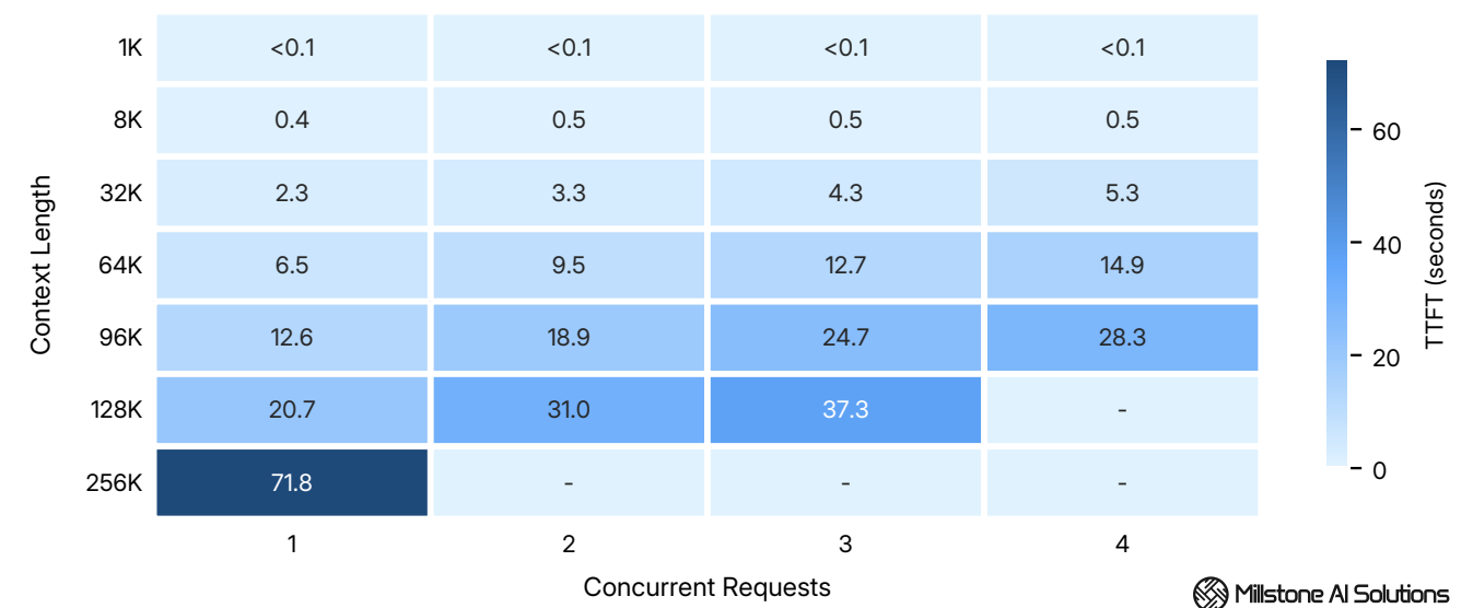
Average time to first token across 1K - 256K tokens context lengths at 1 - 4 concurrency levels.
