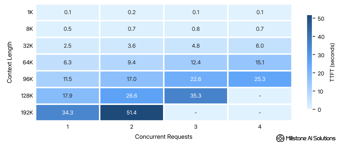
Average time to first token across 1K - 192K tokens context lengths at 1 - 4 concurrency levels.
