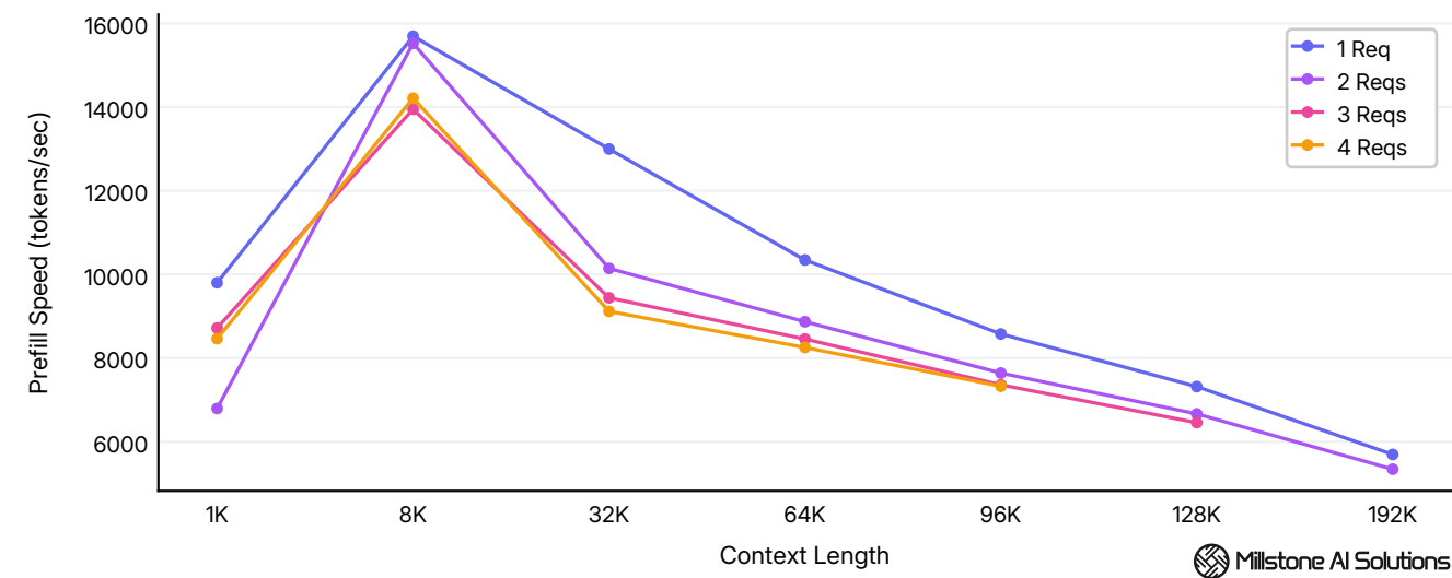
Average per-user prefill speed across 1K - 192K tokens context at 1 - 4 concurrent requests.
