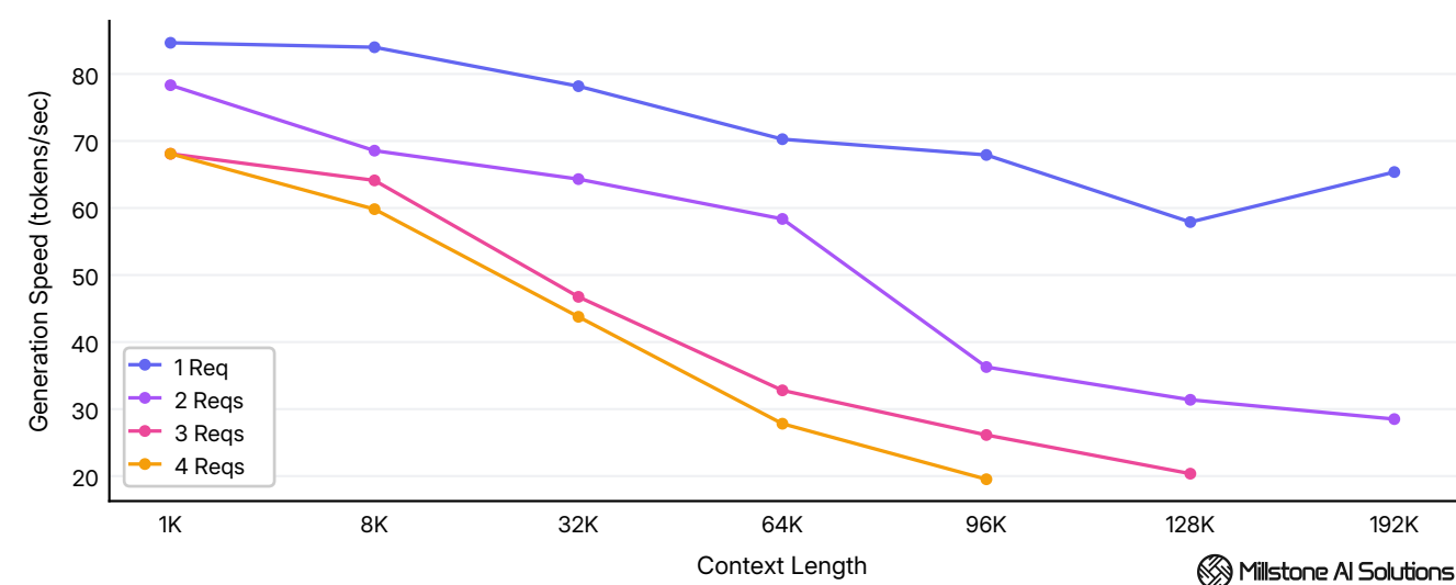
Average per-user generation speed across 1K - 192K tokens context lengths at 1 - 4 concurrency levels.
