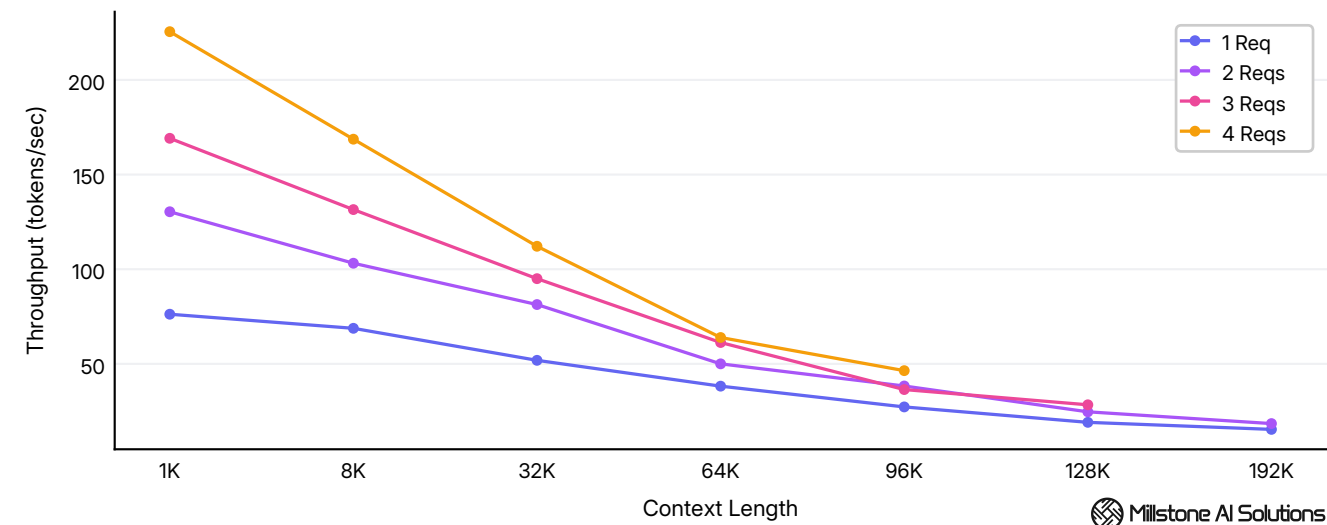
Average system throughput across 1K - 192K tokens context lengths at 1 - 4 concurrency levels.
