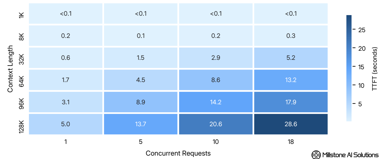
Average time to first token across 1K - 128K tokens context lengths at 1 - 18 concurrency levels.
