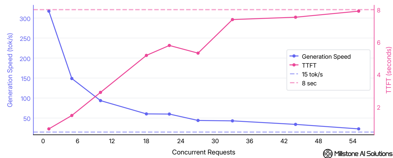
Average per-user generation speed and TTFT at 32K context.
