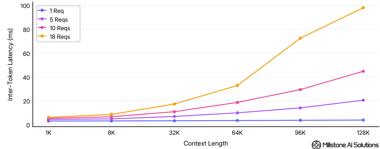
Average inter-token latency across 1K - 128K tokens context at 1 - 18 concurrent requests.
