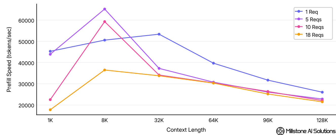
Average per-user prefill speed across 1K - 128K tokens context at 1 - 18 concurrent requests.
