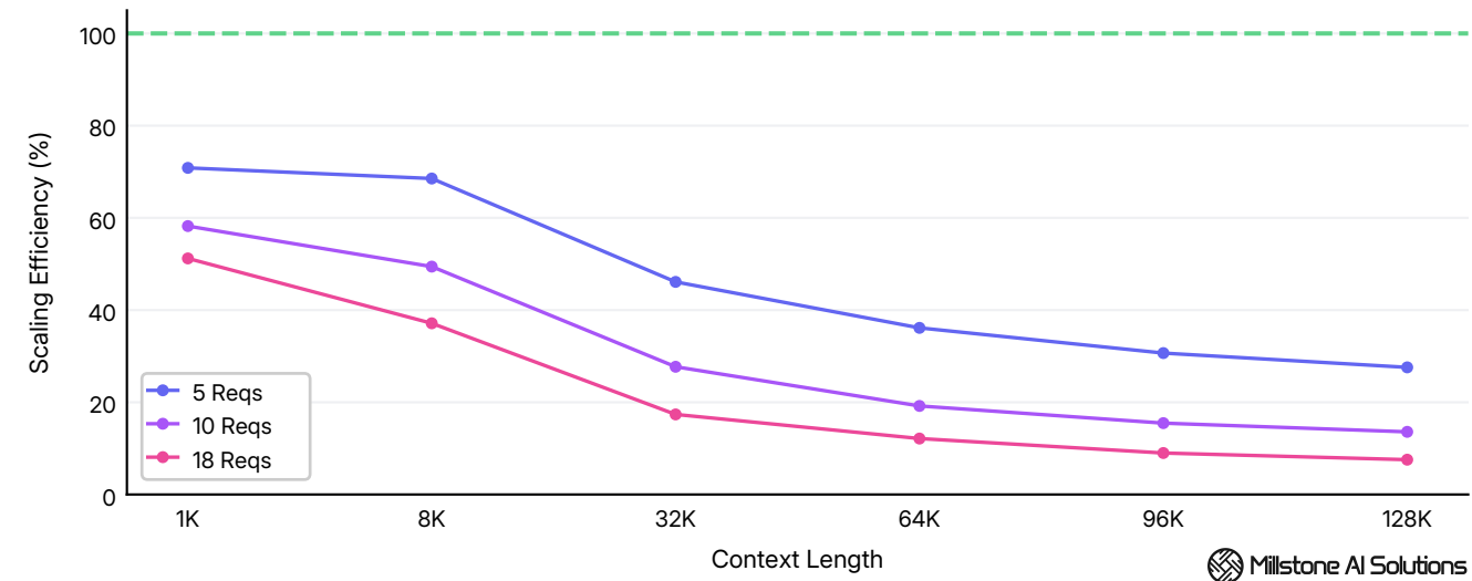
Scaling efficiency across 1K - 128K tokens context at 1 - 18 concurrent requests.
