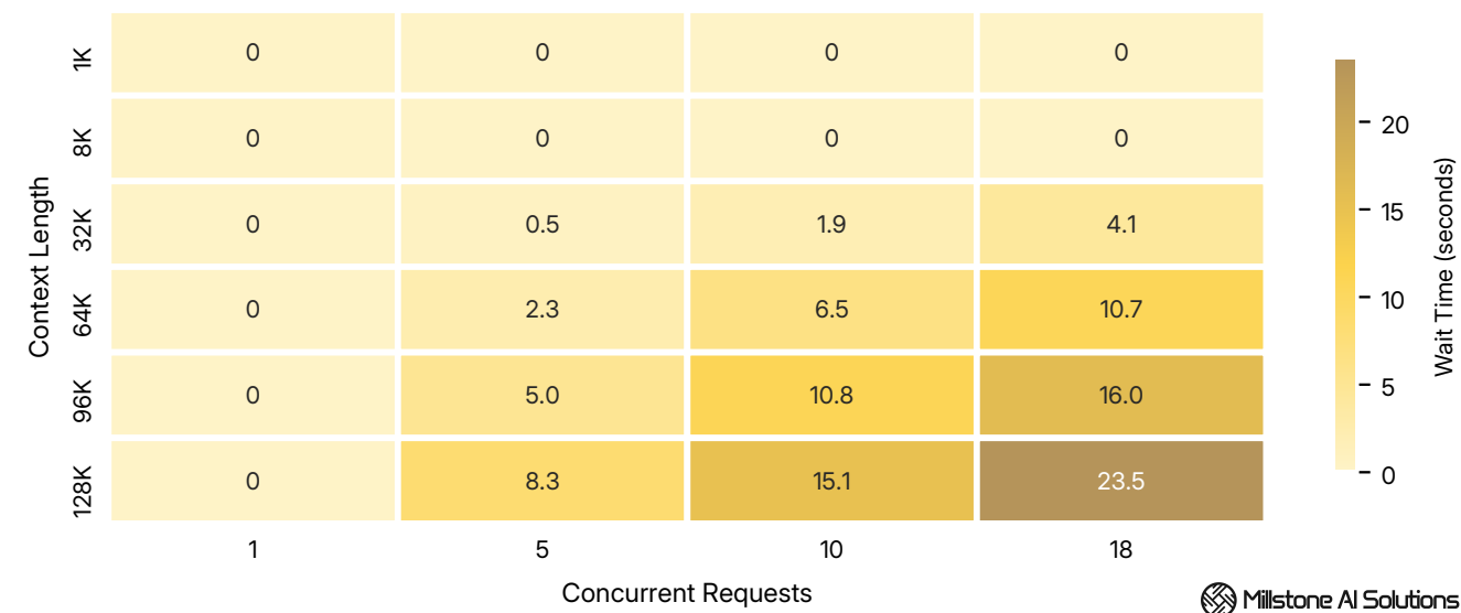
Average queue wait time across 1K - 128K tokens context at 1 - 18 concurrent requests.
