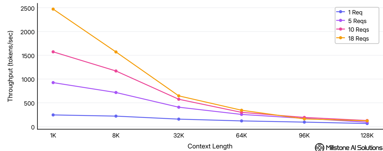
Average system throughput across 1K - 128K tokens context lengths at 1 - 18 concurrency levels.
