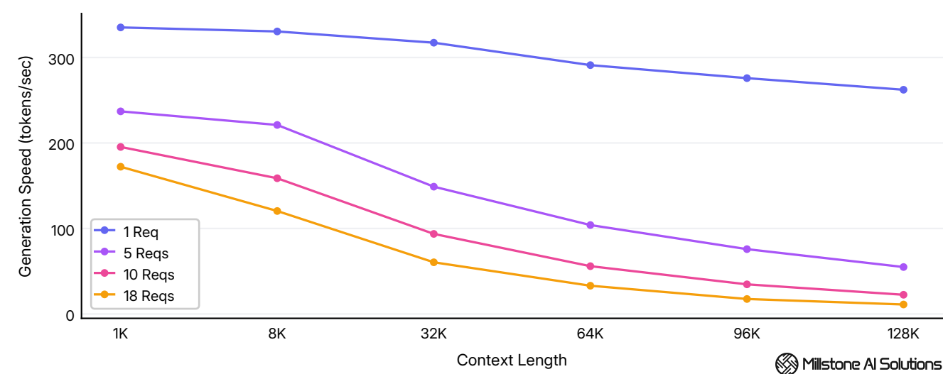
Average per-user generation speed across 1K - 128K tokens context lengths at 1 - 18 concurrency levels.
