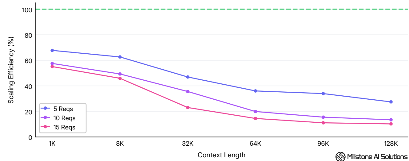
Scaling efficiency across 1K - 128K tokens context at 1 - 15 concurrent requests.
