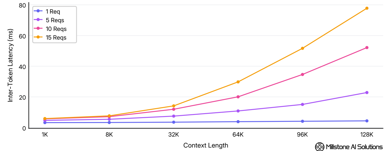
Average inter-token latency across 1K - 128K tokens context at 1 - 15 concurrent requests.
