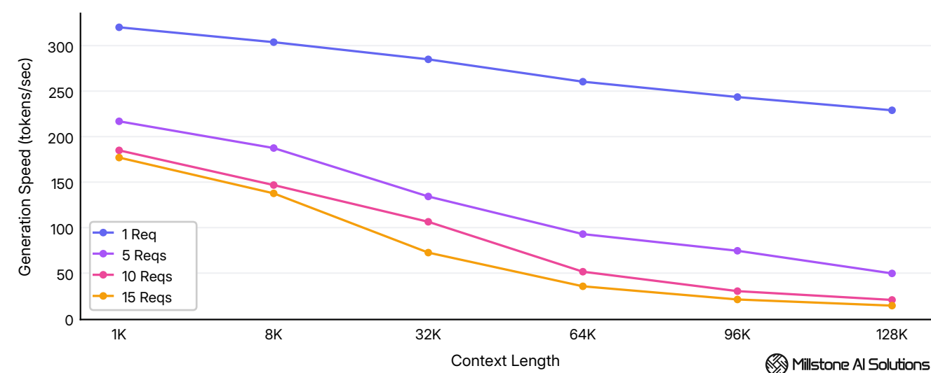
Average per-user generation speed across 1K - 128K tokens context lengths at 1 - 15 concurrency levels.
