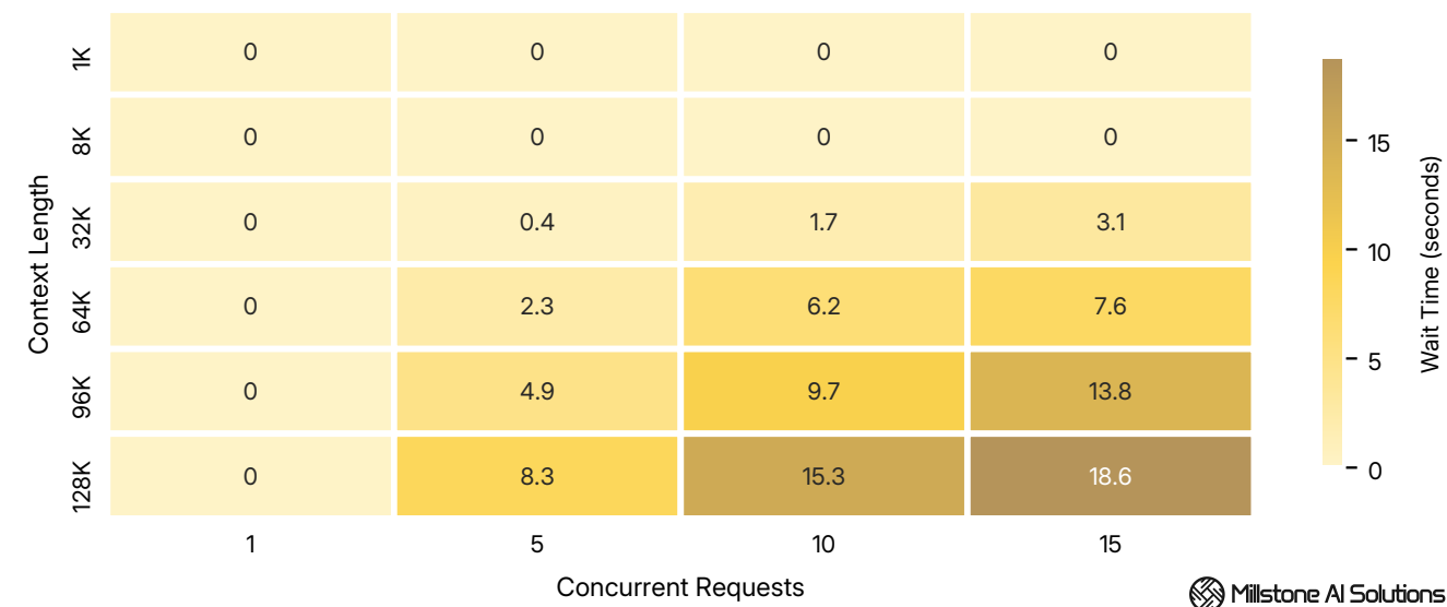
Average queue wait time across 1K - 128K tokens context at 1 - 15 concurrent requests.
