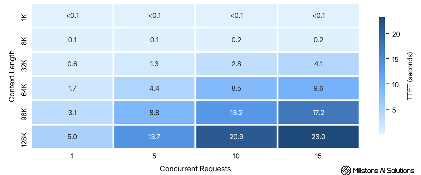
Average time to first token across 1K - 128K tokens context lengths at 1 - 15 concurrency levels.
