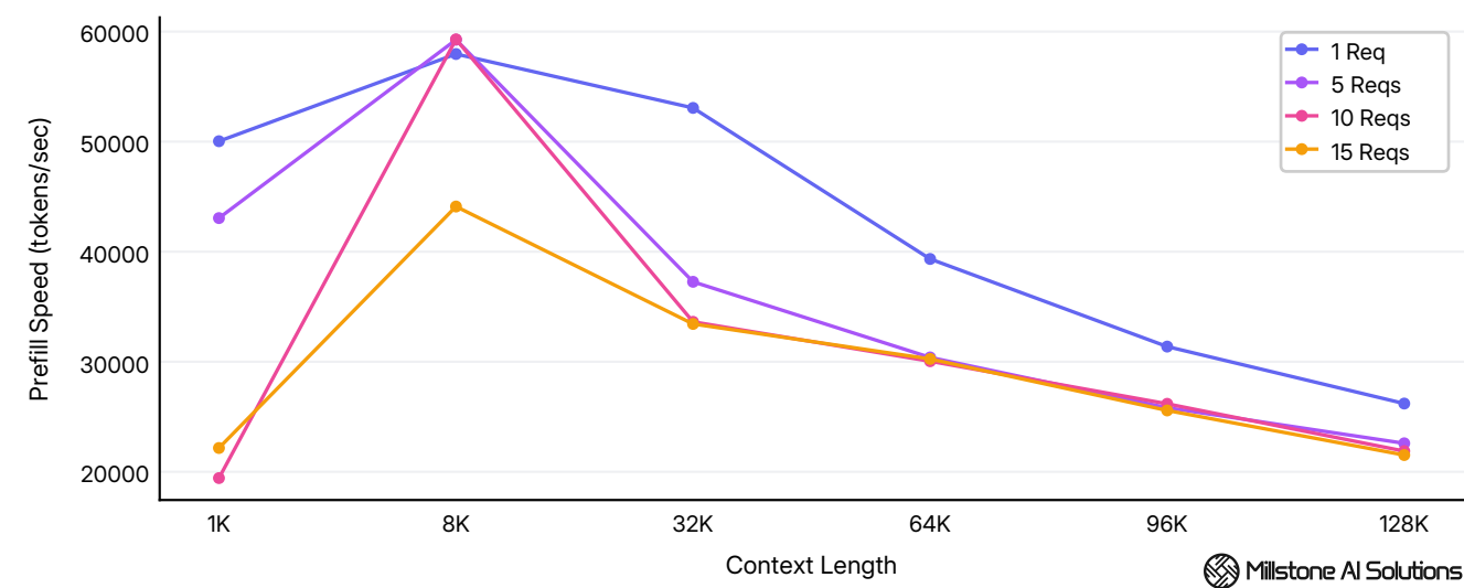
Average per-user prefill speed across 1K - 128K tokens context at 1 - 15 concurrent requests.
