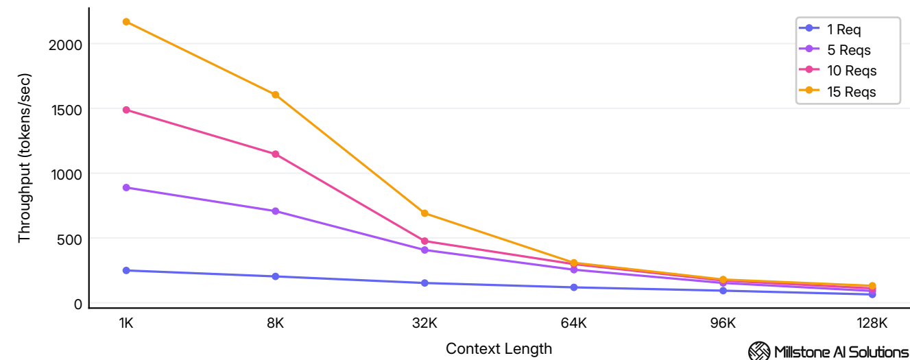
Average system throughput across 1K - 128K tokens context lengths at 1 - 15 concurrency levels.
