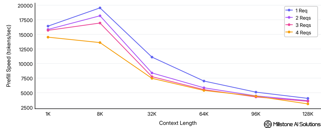
Average per-user prefill speed across 1K - 128K tokens context at 1 - 4 concurrent requests.
