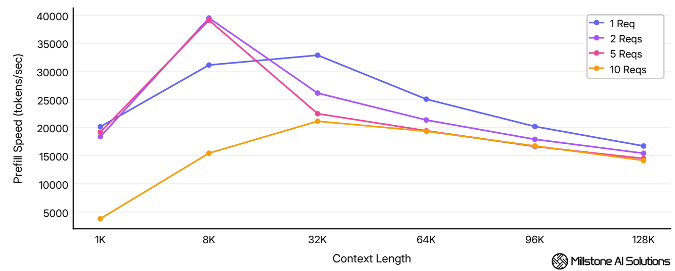
Average per-user prefill speed across 1K - 128K tokens context at 1 - 10 concurrent requests.
