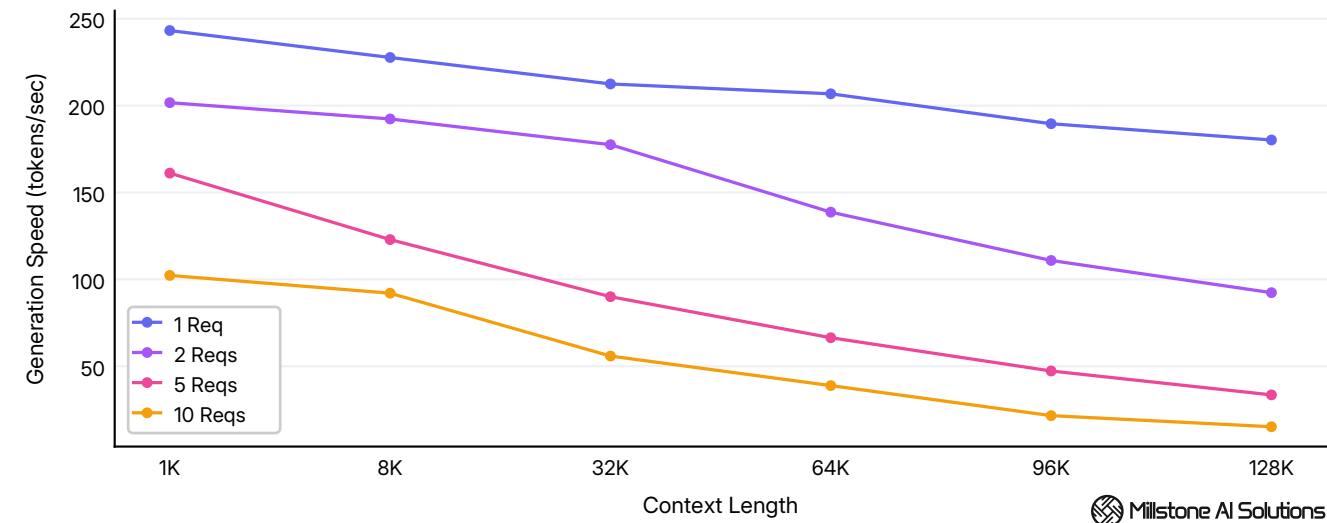
Average per-user generation speed across 1K - 128K tokens context lengths at 1 - 10 concurrency levels.
