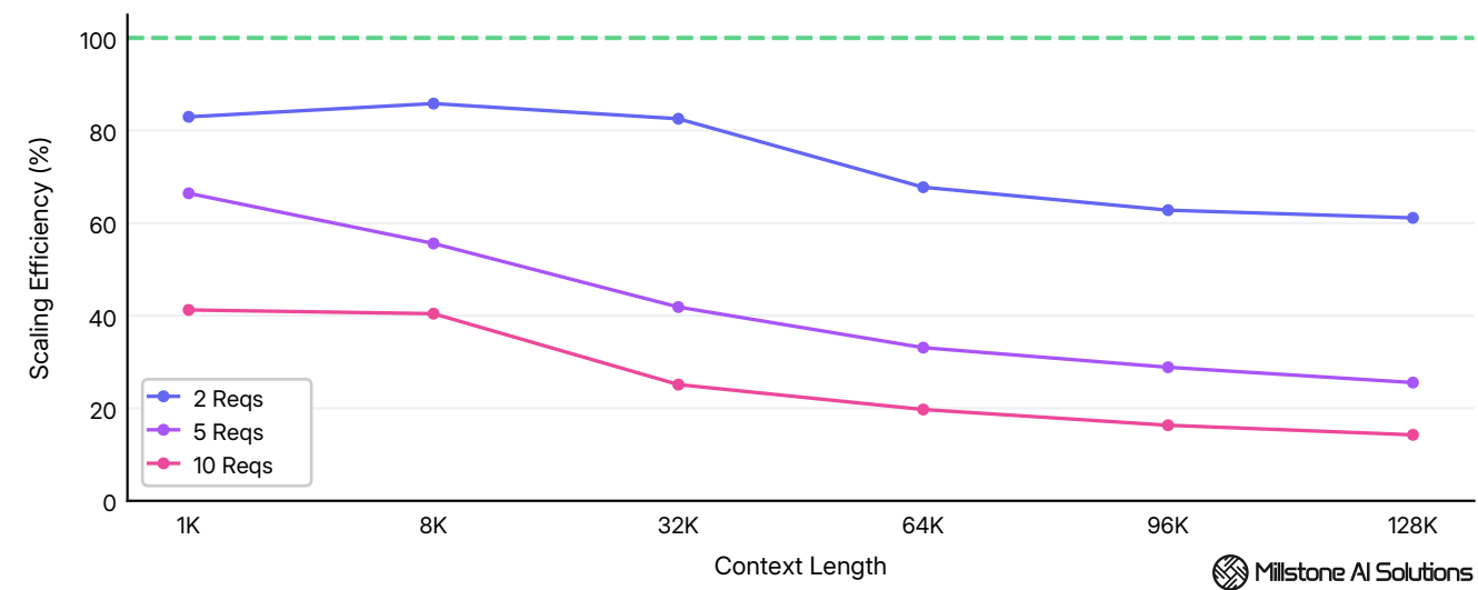
Scaling efficiency across 1K - 128K tokens context at 1 - 10 concurrent requests.
