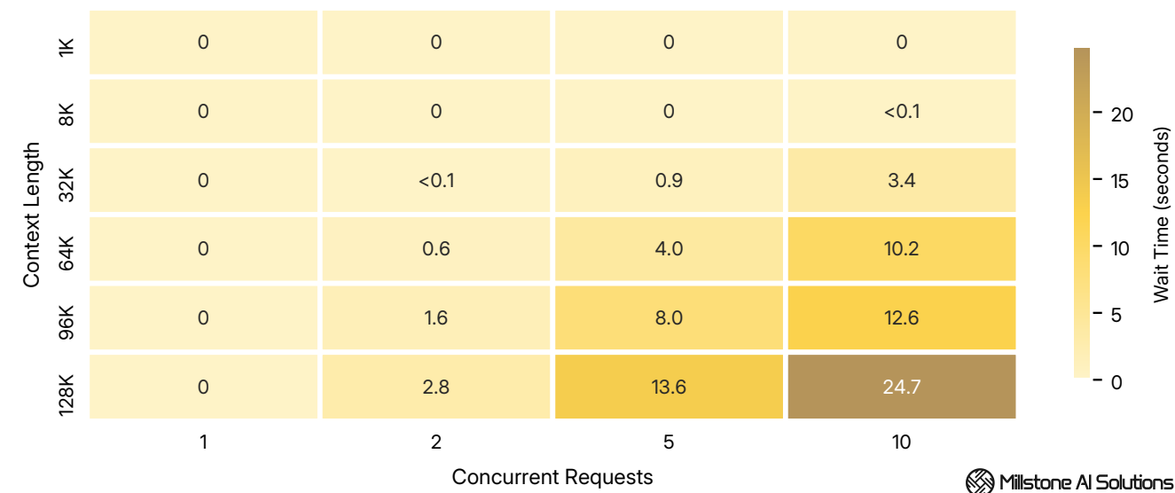
Average queue wait time across 1K - 128K tokens context at 1 - 10 concurrent requests.
