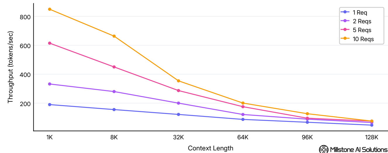
Average system throughput across 1K - 128K tokens context lengths at 1 - 10 concurrency levels.
