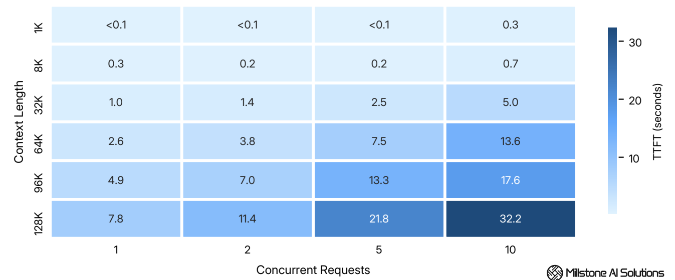
Average time to first token across 1K - 128K tokens context lengths at 1 - 10 concurrency levels.
