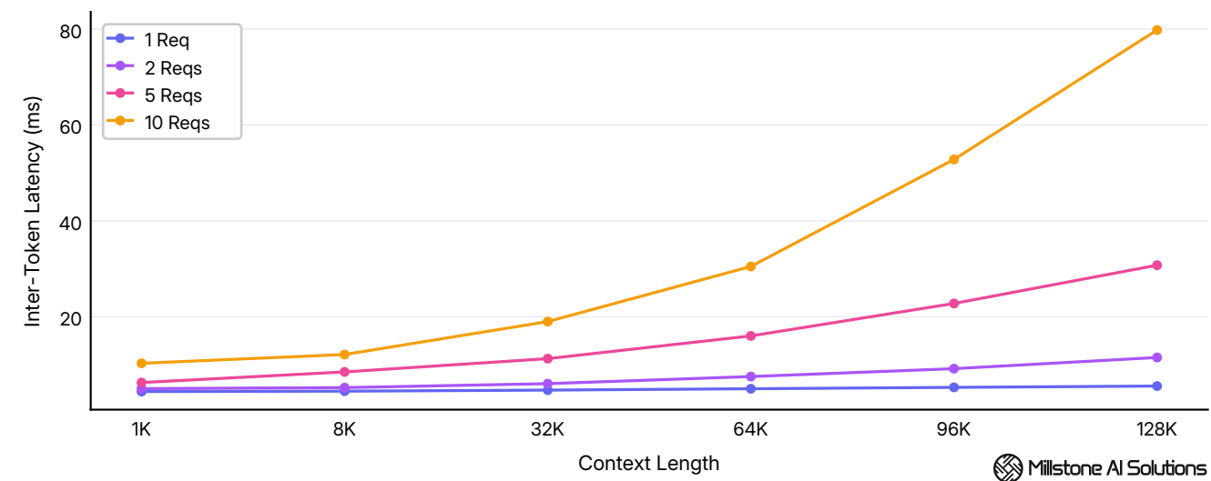
Average inter-token latency across 1K - 128K tokens context at 1 - 10 concurrent requests.
