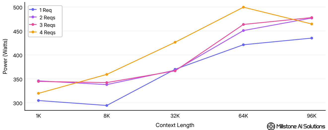
Average GPU power draw across 1K - 96K tokens context at 1 - 4 concurrent requests.
