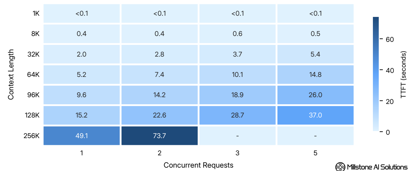
Average time to first token across 1K - 256K tokens context lengths at 1 - 5 concurrency levels.
