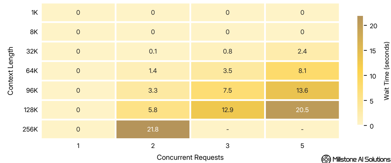
Average queue wait time across 1K - 256K tokens context at 1 - 5 concurrent requests.
