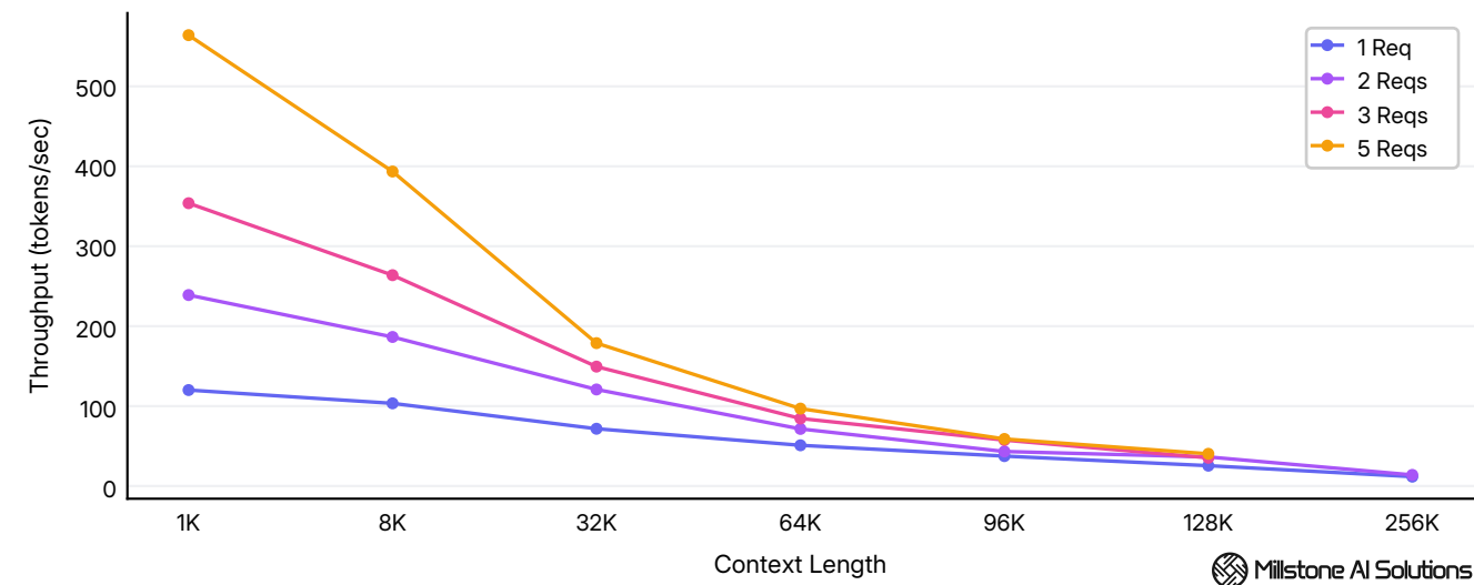
Average system throughput across 1K - 256K tokens context lengths at 1 - 5 concurrency levels.
