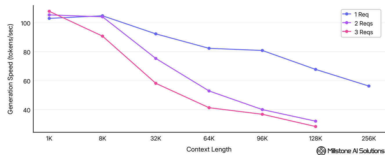
Average per-user generation speed across 1K - 256K tokens context lengths at 1 - 3 concurrency levels.
