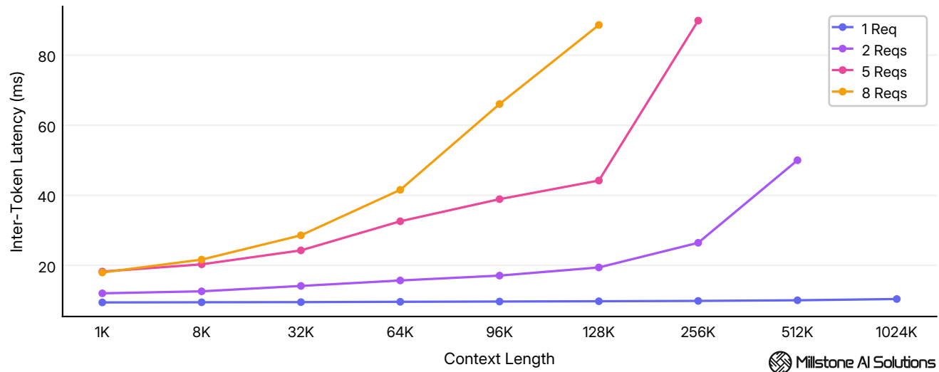
Average inter-token latency across 1K - 1024K tokens context at 1 - 8 concurrent requests.
