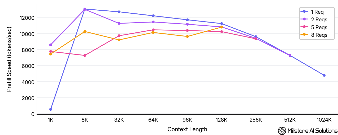
Average per-user prefill speed across 1K - 1024K tokens context at 1 - 8 concurrent requests.
