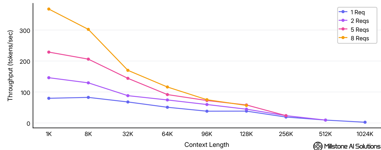
Average system throughput across 1K - 1024K tokens context lengths at 1 - 8 concurrency levels.
