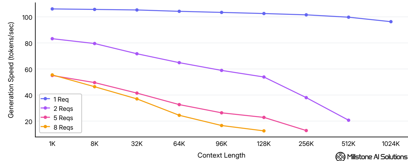
Average per-user generation speed across 1K - 1024K tokens context lengths at 1 - 8 concurrency levels.
