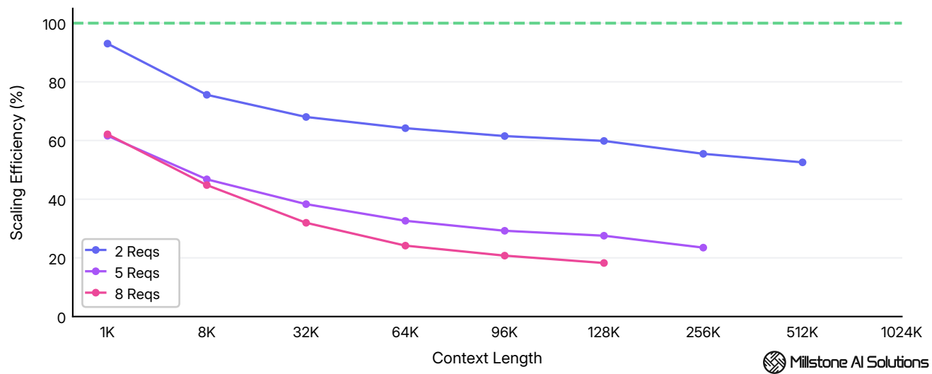
Scaling efficiency across 1K - 512K tokens context at 1 - 8 concurrent requests.
